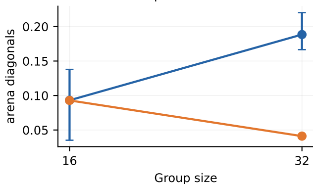
Predator | Predator distance
