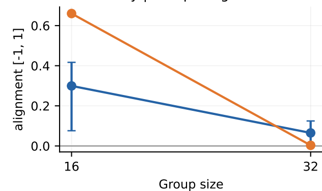
Prey | Escape alignment
