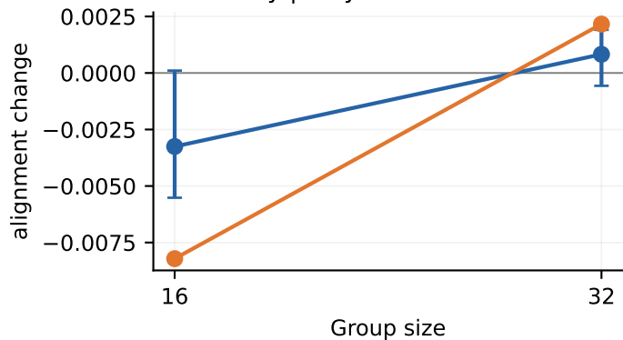
Prey | Prey reorientation R
