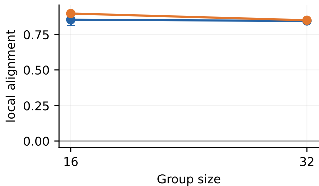
Collective | DoA (T-common)
