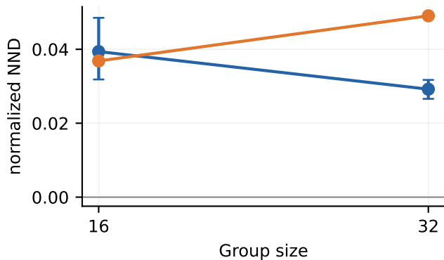
Collective | DoS (T-common)
